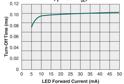
Typical Turn-Off Time vs. LED Forward Current (I F =150mA DC )
